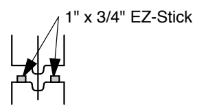
Typical Tongue & Groove Joint
