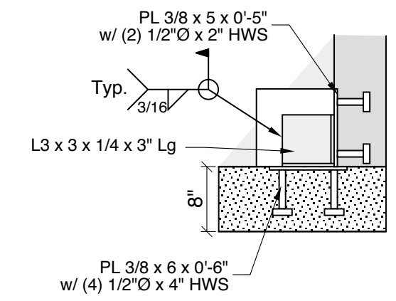
Typ. Weld Plate Detail
