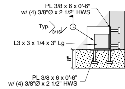
Typ. Weld Plate Detail
