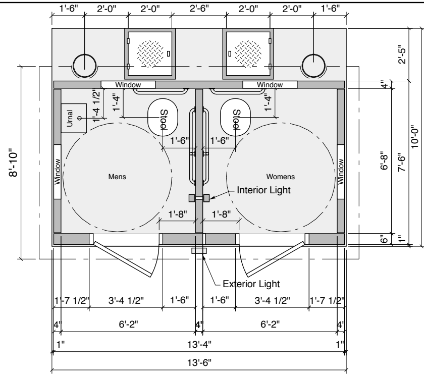
Plan View
