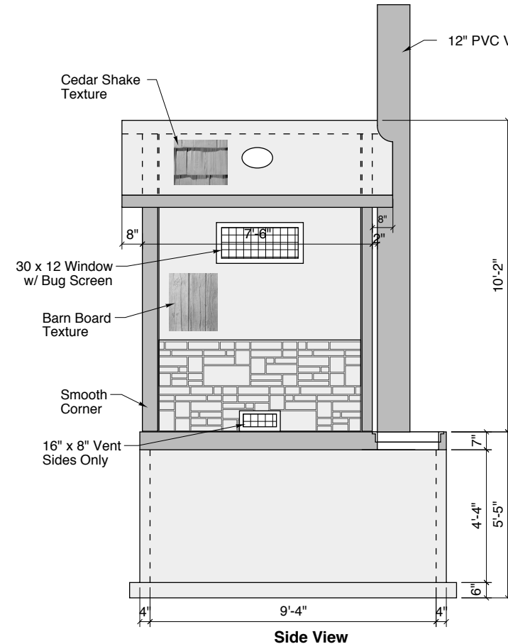
Side View
