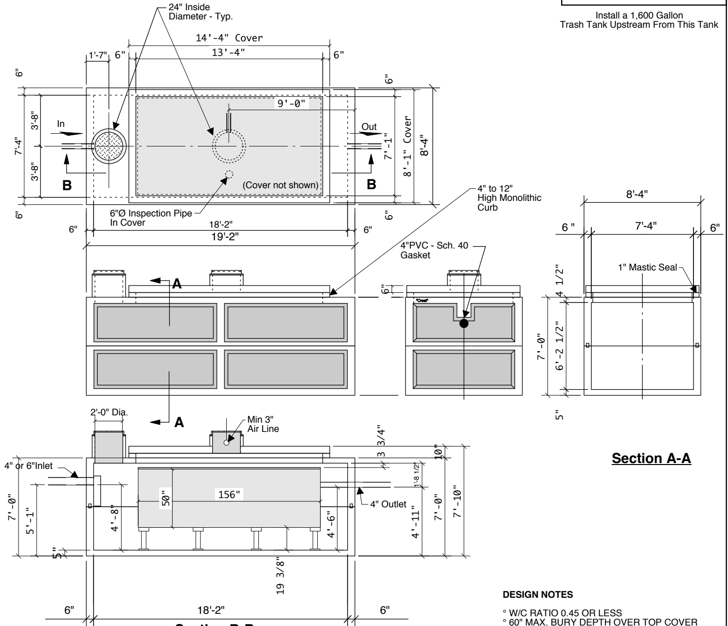
Section B-B
