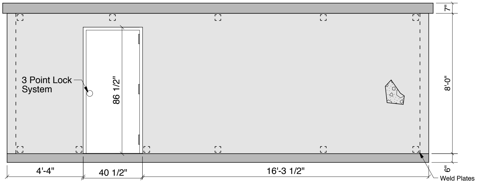
Front Elevation
