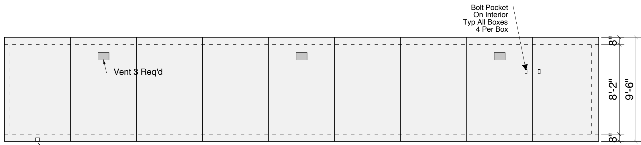
Front View
