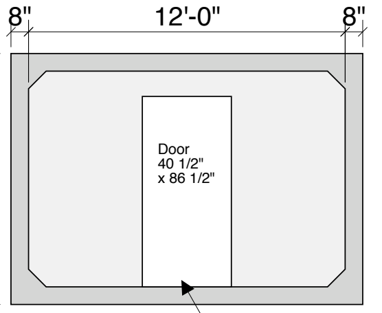
End View
